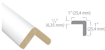
90° Corner Moulding 4439
