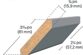
O'gee KA
