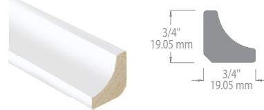
Cove Moulding 4786
