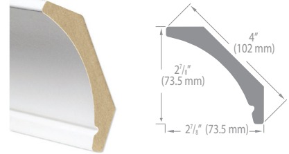
Contemporary O'Gee 4766
